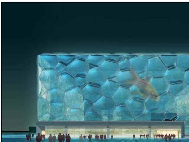
Ethylene-tetra-flouro-ethylene (ETFE)
